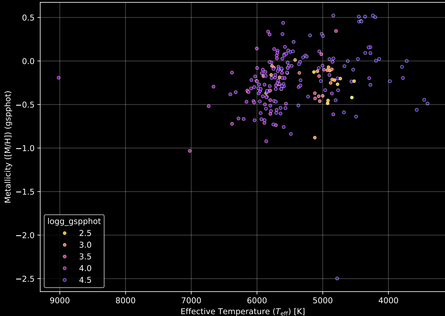
APOGEE DR17 Field: [110+64_MGA] Stellar Population Parameters (n= 207)
