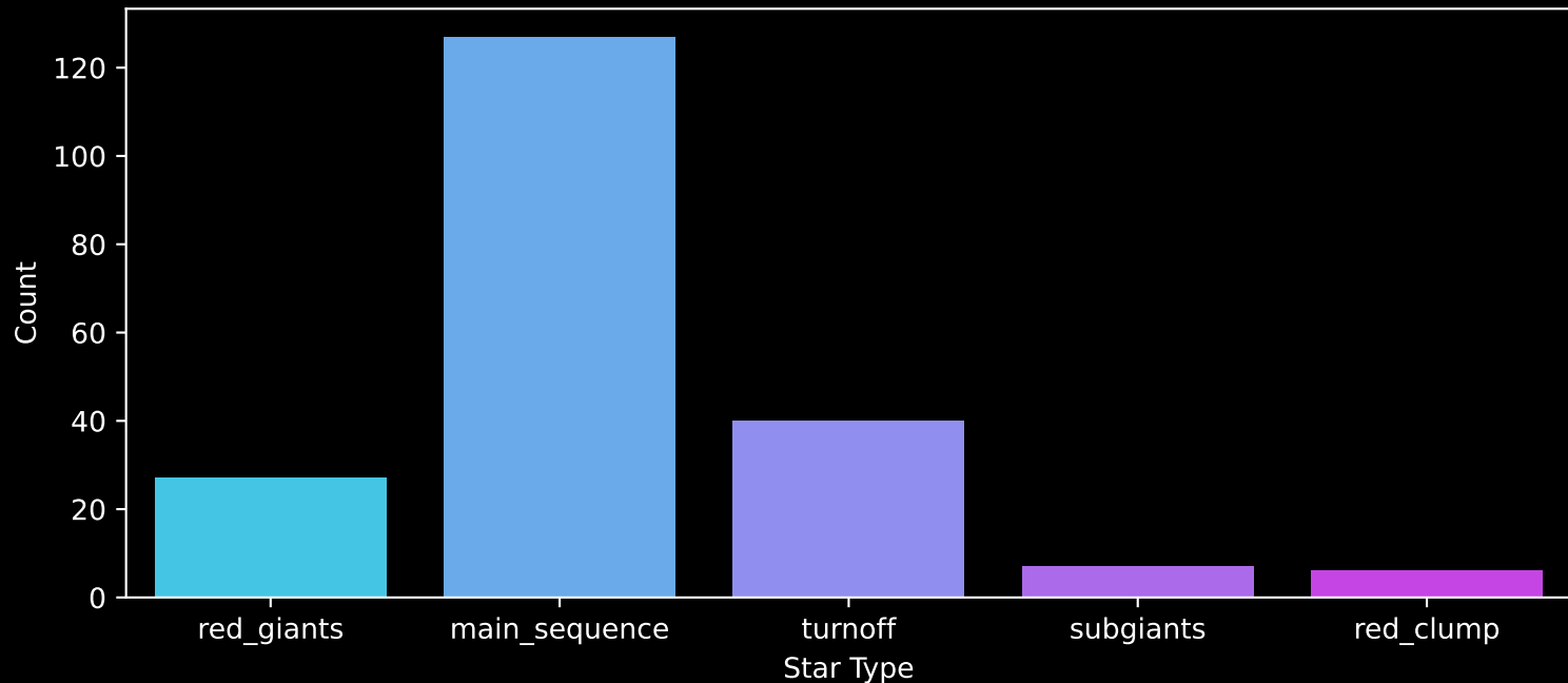
APOGEE DR17 Field: [110+64_MGA] Count plot of Star Type
