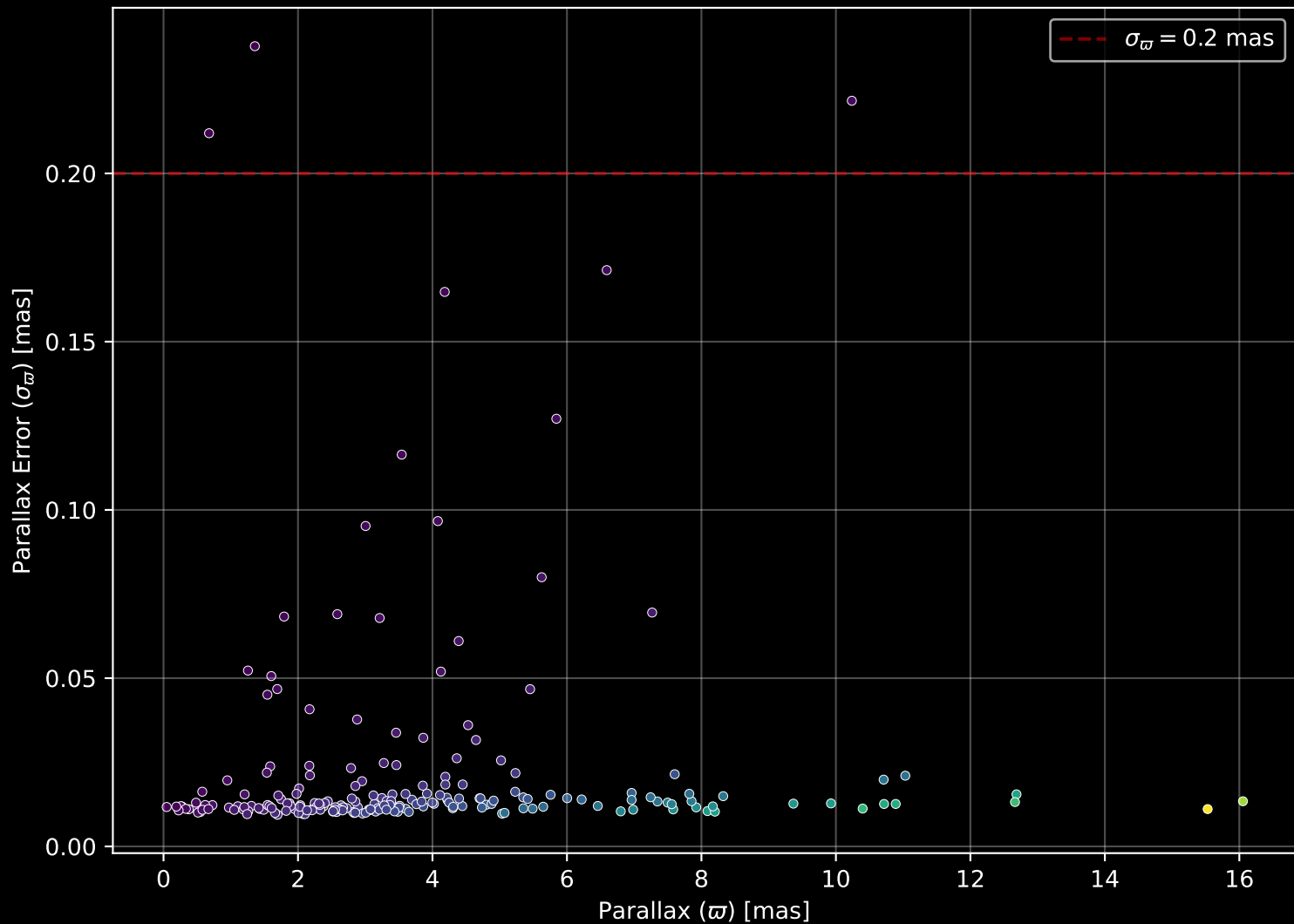
APOGEE DR17 Field: [110+64_MGA] Parallax Quality (n= 207)
