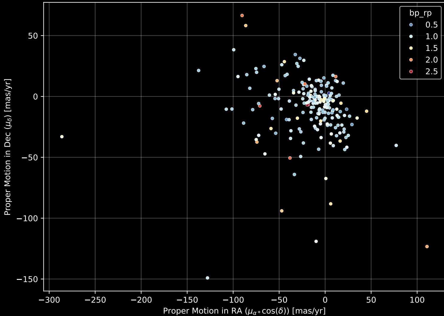
APOGEE DR17 Field: [110+64_MGA] Proper Motion Diagram (n= 207)
